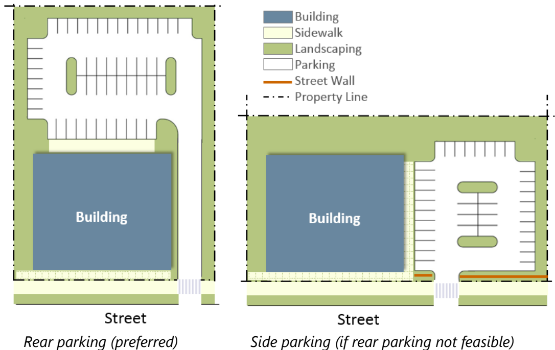
Figure VIII - 51: Parking Location
