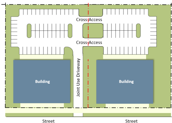
Figure VIII - 48: Joint Use Driveways/Cross-Access.
