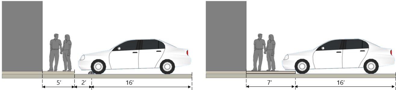
Figure VIII - 52: Parking Overhang
